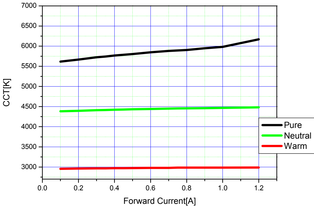
CCT vs. Forward Current, Ta=25°C
