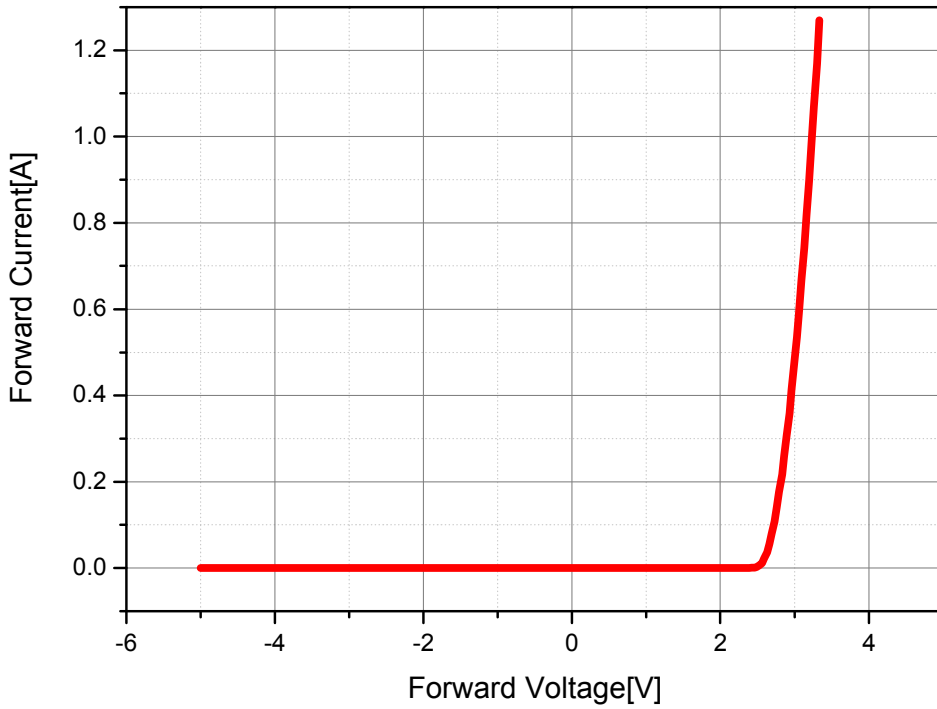
Forward Voltage vs. Forward Current, Ta=25℃
